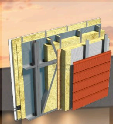
DETALIU FATADA
