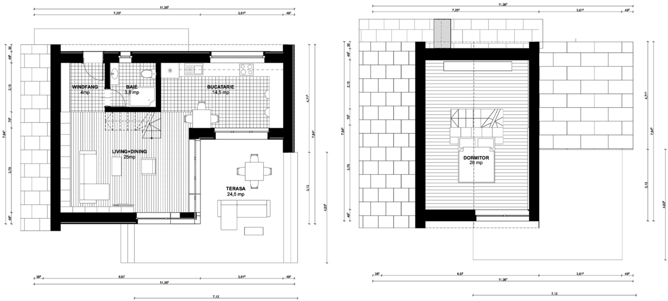
PLAN PARTER
