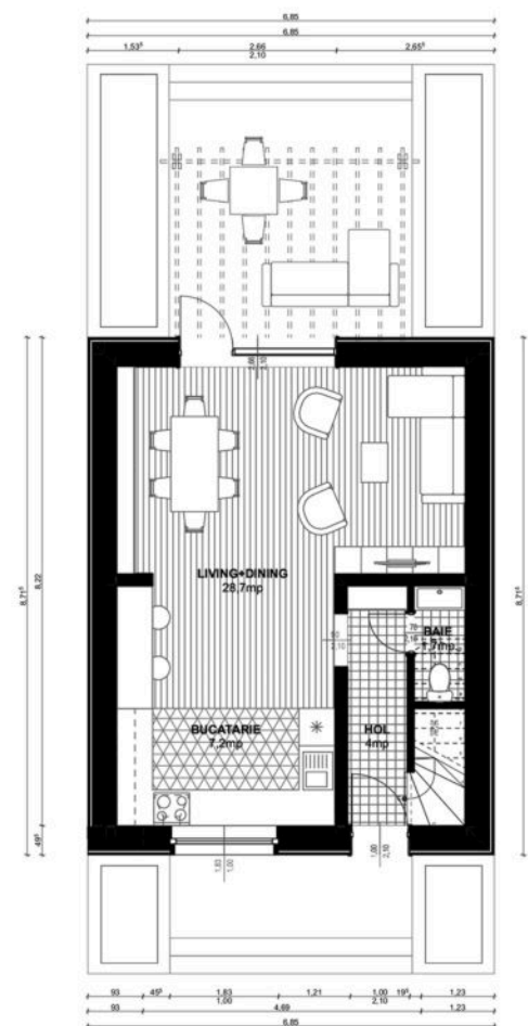
PLAN PARTER
