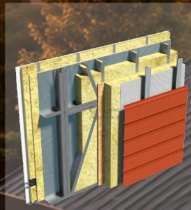
DETALIU FATADA
