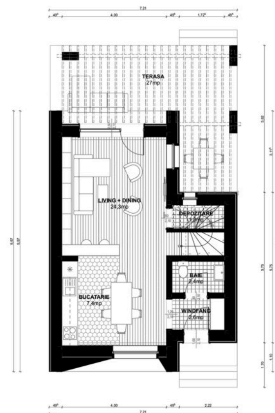
PLAN PARTER
